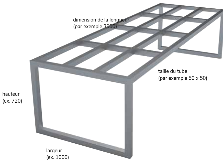
Structure Lampione-3000
