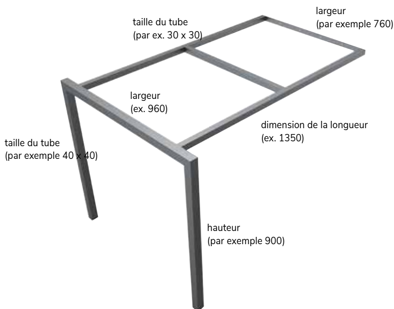
Structure Linosa-1500
