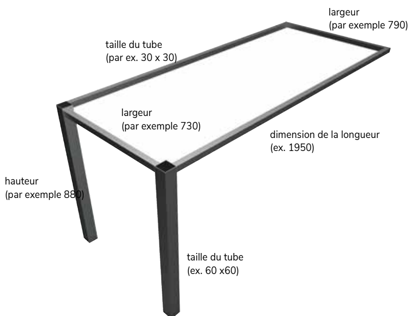
Structure Levanzo-2000
