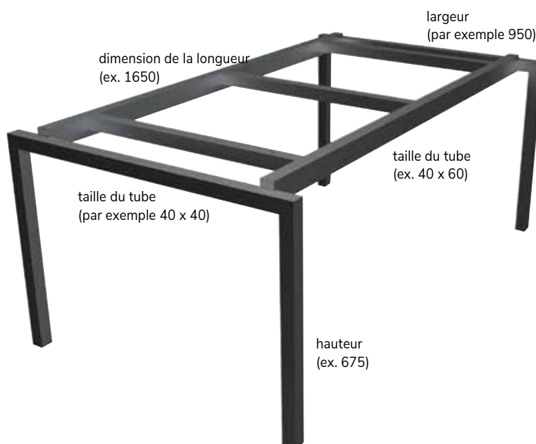
Structure Torcello-2000
